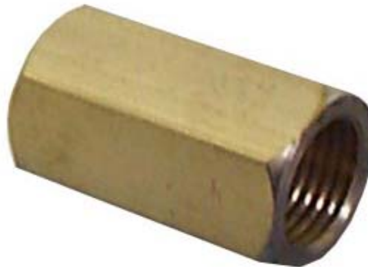
1/4-27 Male by 7/16-24 Female Brass Adapter 24C0-21M-31F
